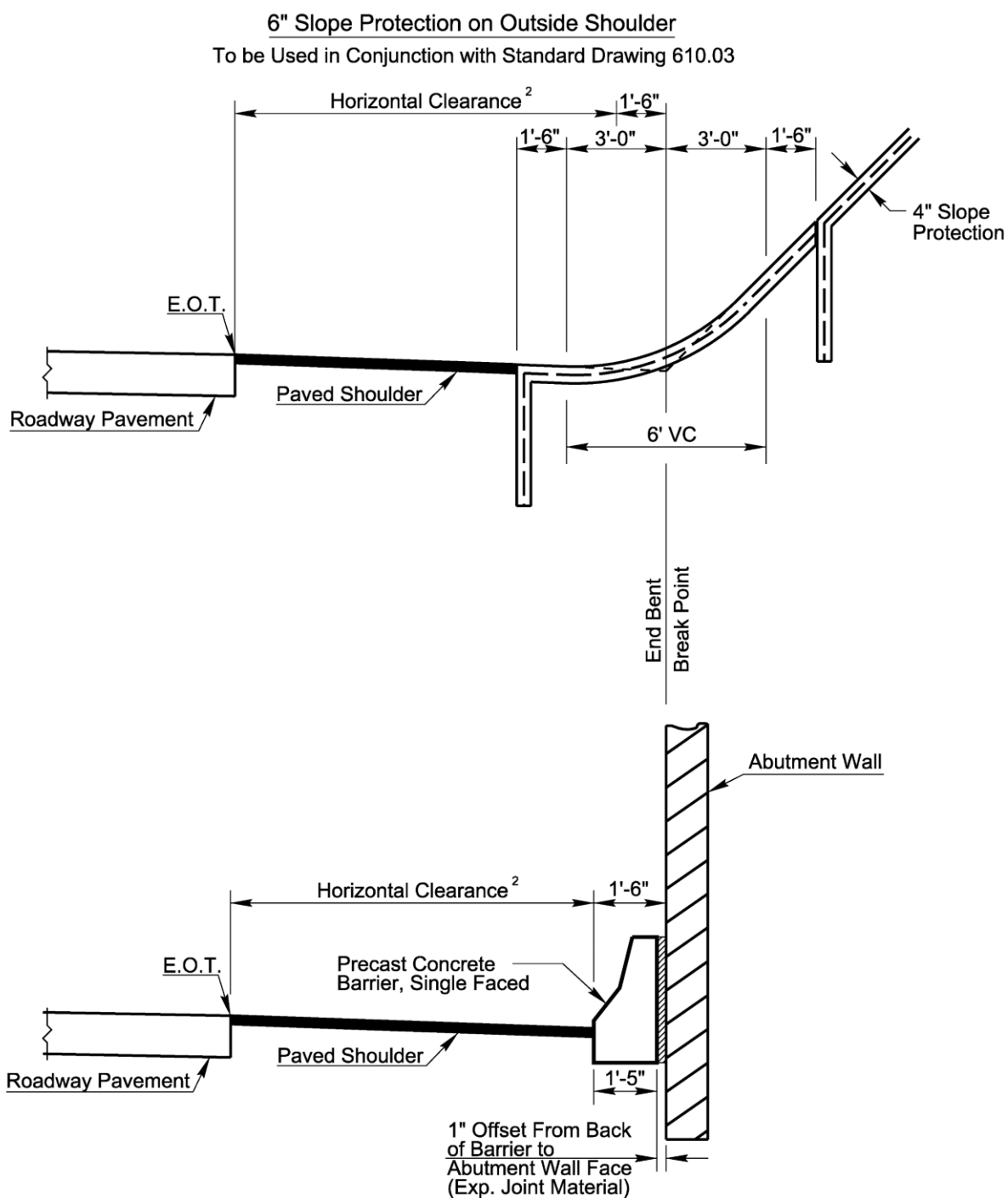
Figure 5-22 Shoulder Detail Under Bridge with 6-Inch Slope Protection or Abutment Wall
